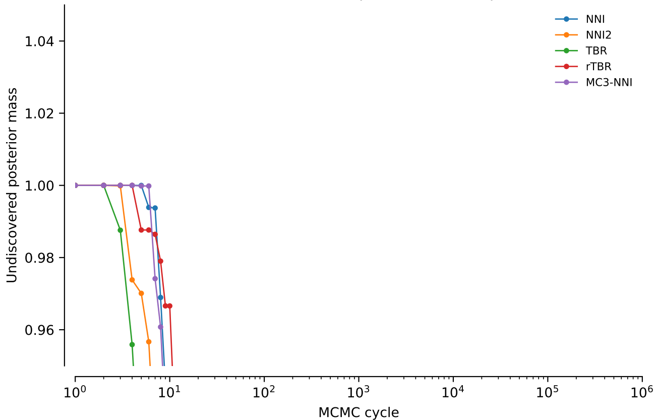
vert.coiii.tw2: Undiscovered posterior mass: power = 0.2
