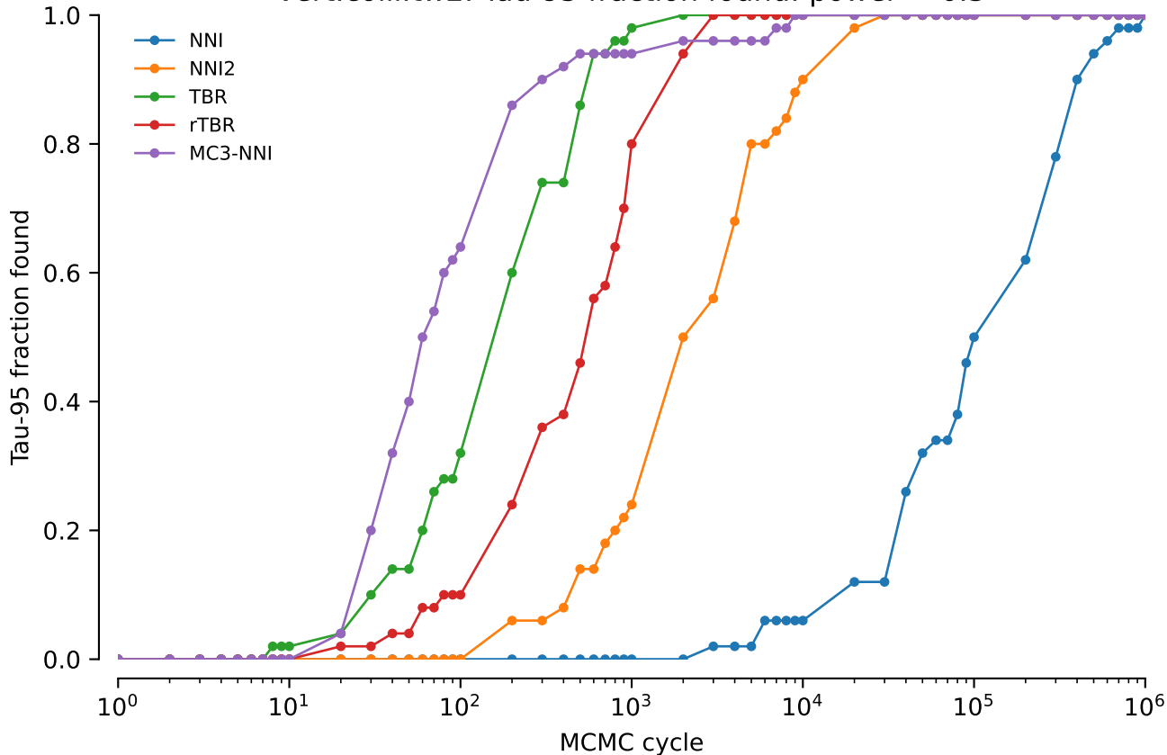
vert.coiii.tw2: Tau-95 fraction found: power = 0.3
