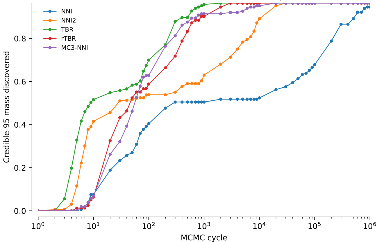
vert.coiii.tw2: Credible-95 mass discovered: power = 0.4
