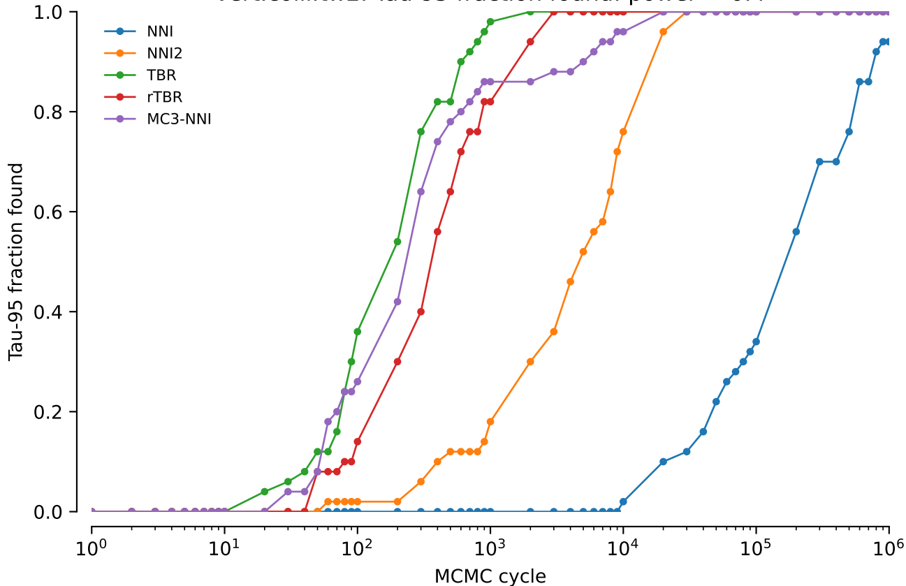
vert.coiii.tw2: Tau-95 fraction found: power = 0.4
