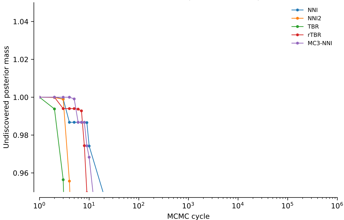
vert.coiii.tw2: Undiscovered posterior mass: power = 0.5
