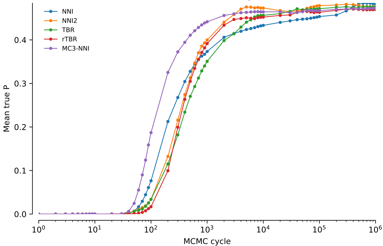
vert.coiii.tw2: Mean true P: power = 0
