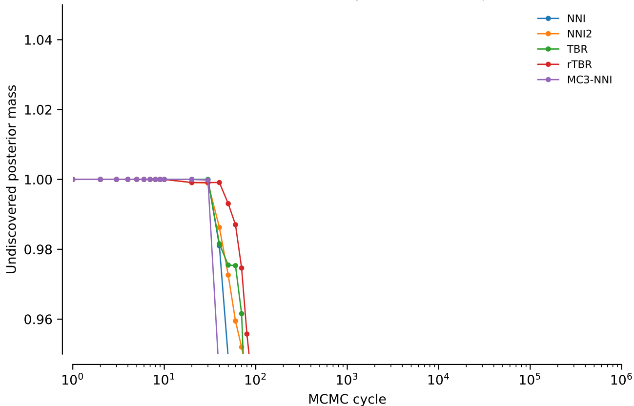
vert.coiii.tw2: Undiscovered posterior mass: power = 0
