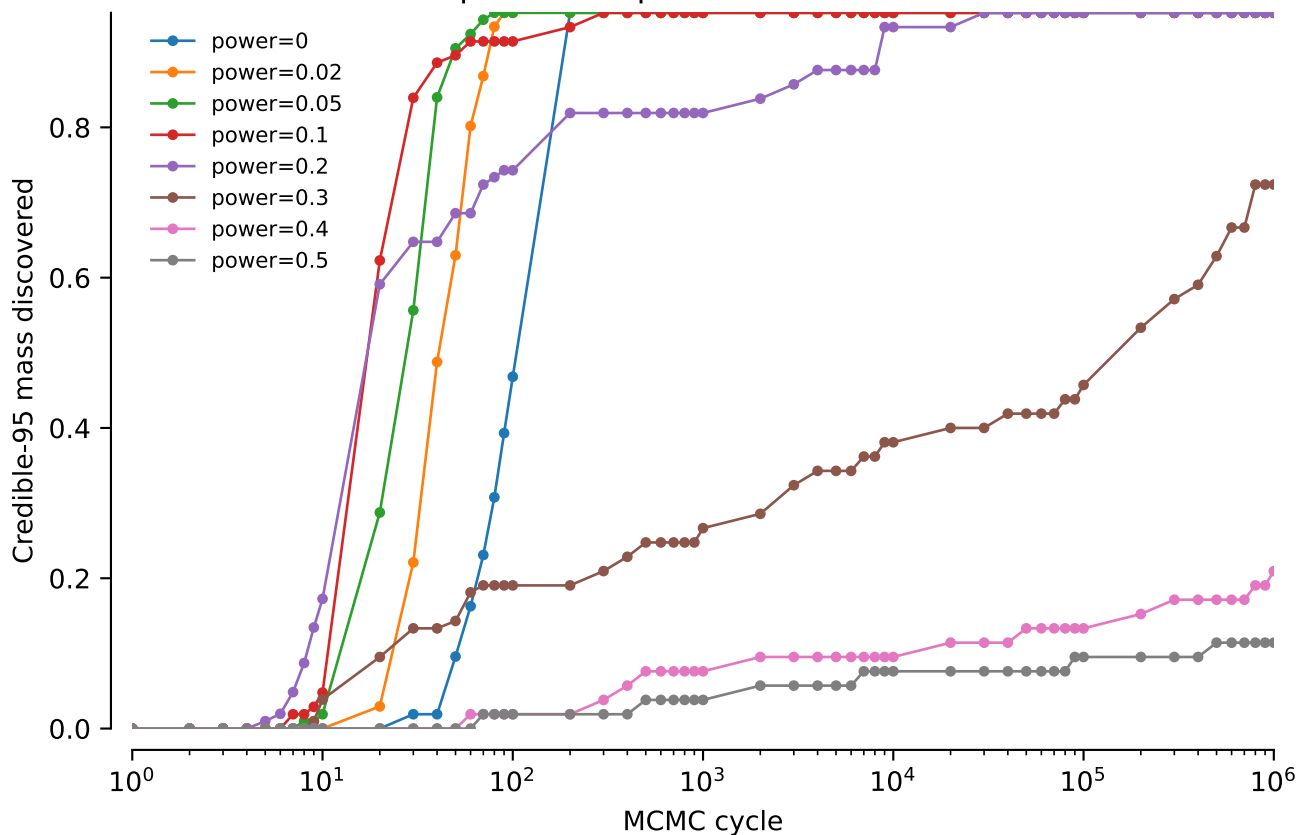
vert.nd1.tw0: NNI power comparison: Credible-95 mass discovered
