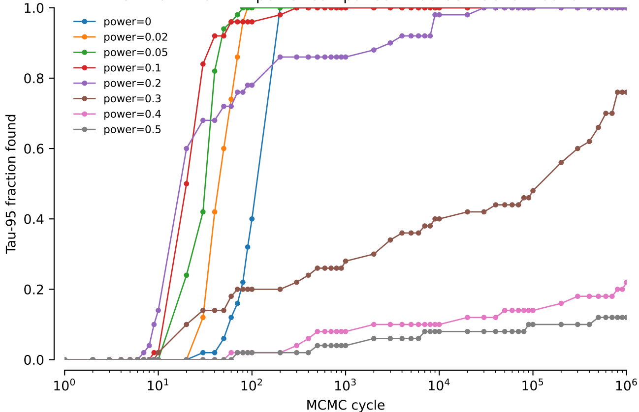
vert.nd1.tw0: NNI power comparison: Tau-95 fraction found
