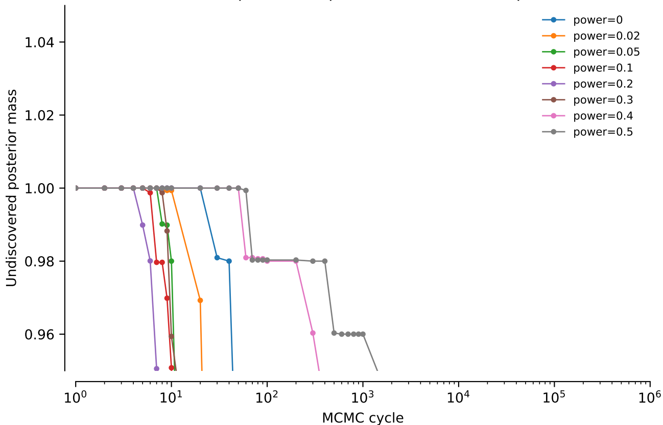
vert.nd1.tw0: NNI power comparison: Undiscovered posterior mass
