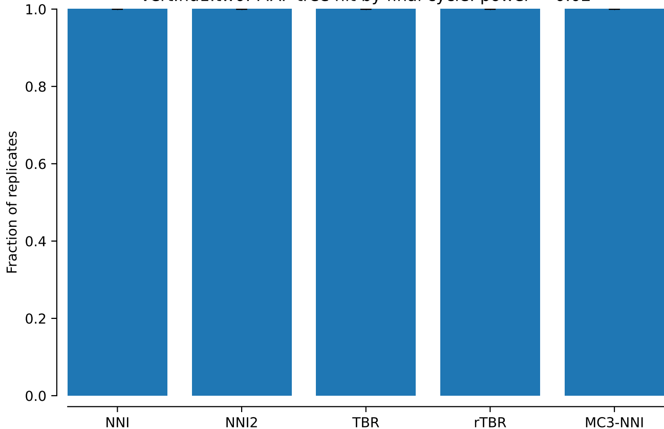
vert.nd1.tw0: MAP tree hit by final cycle: power = 0.02
