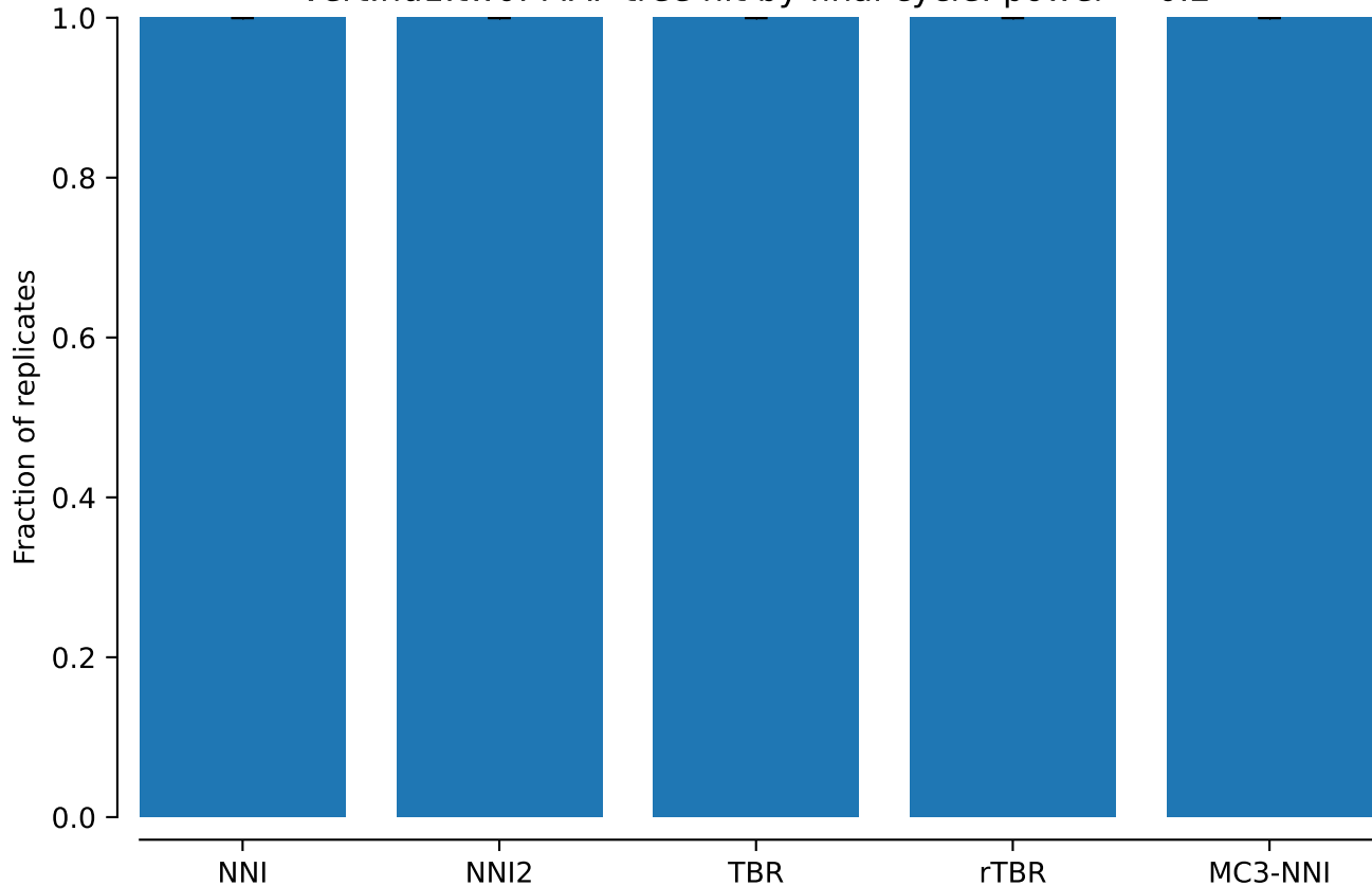
vert.nd1.tw0: MAP tree hit by final cycle: power = 0.2
