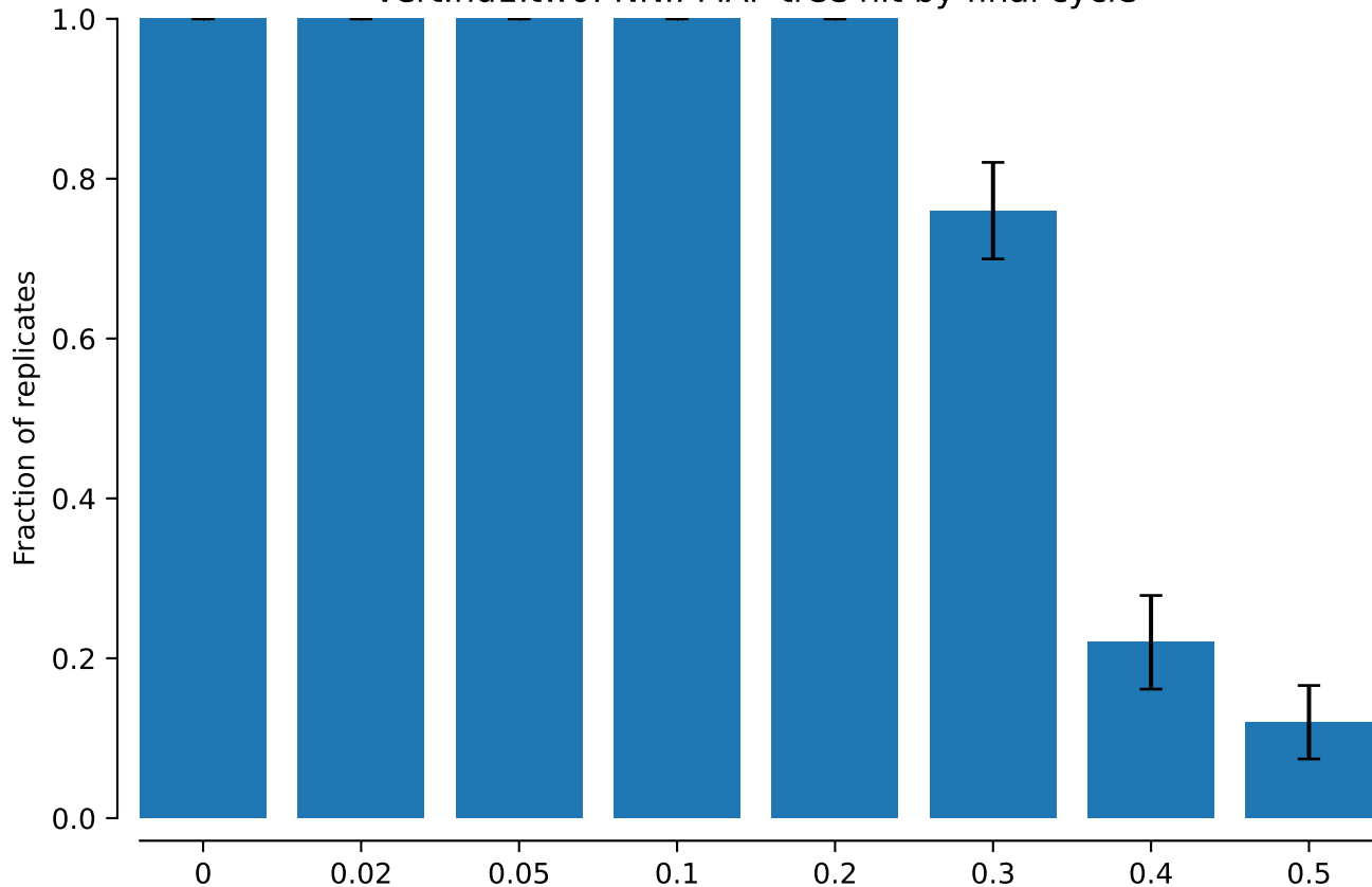
vert.nd1.tw0: NNI: MAP tree hit by final cycle
