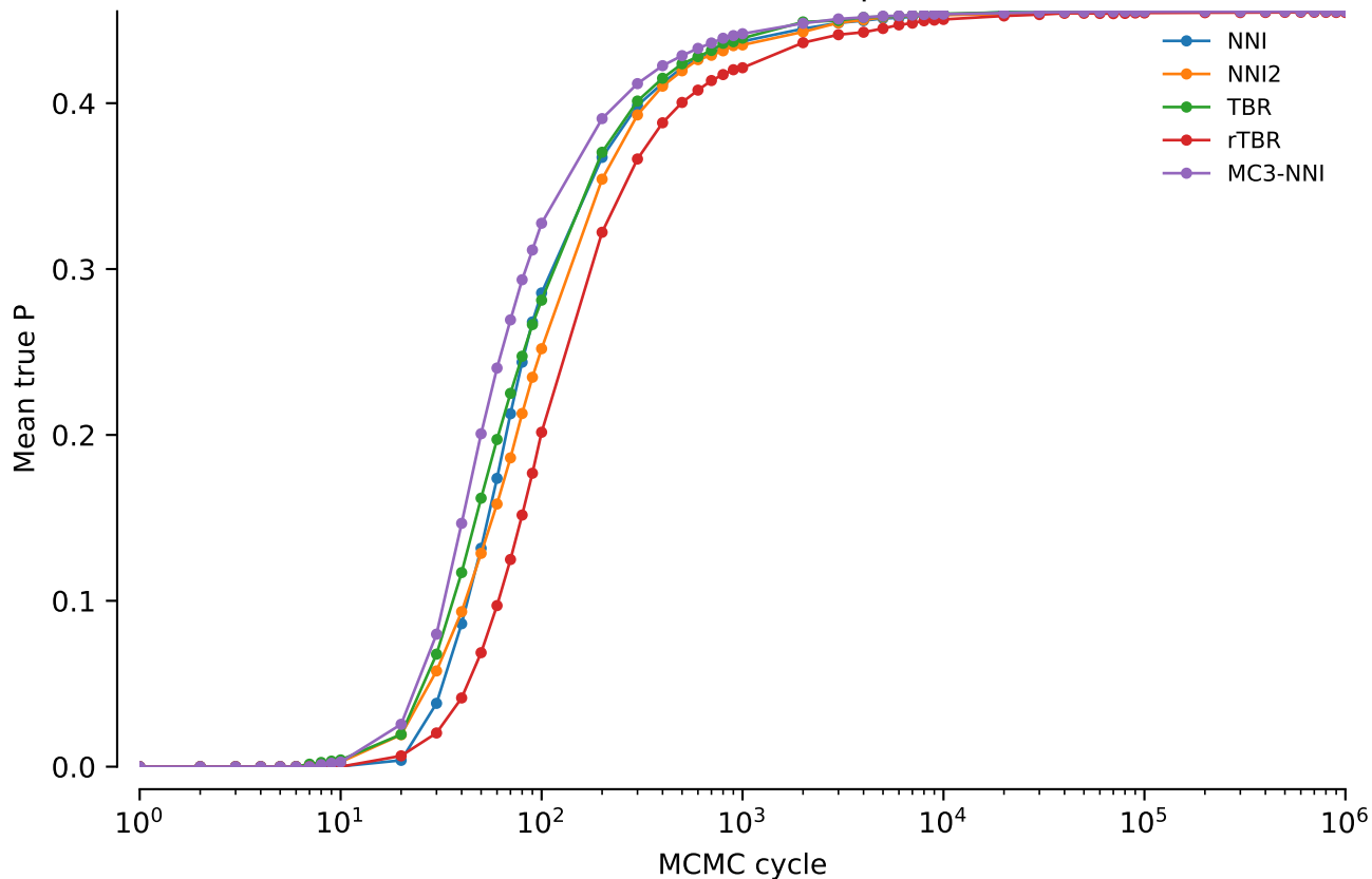
vert.nd1.tw0: Mean true P: power = 0.02
