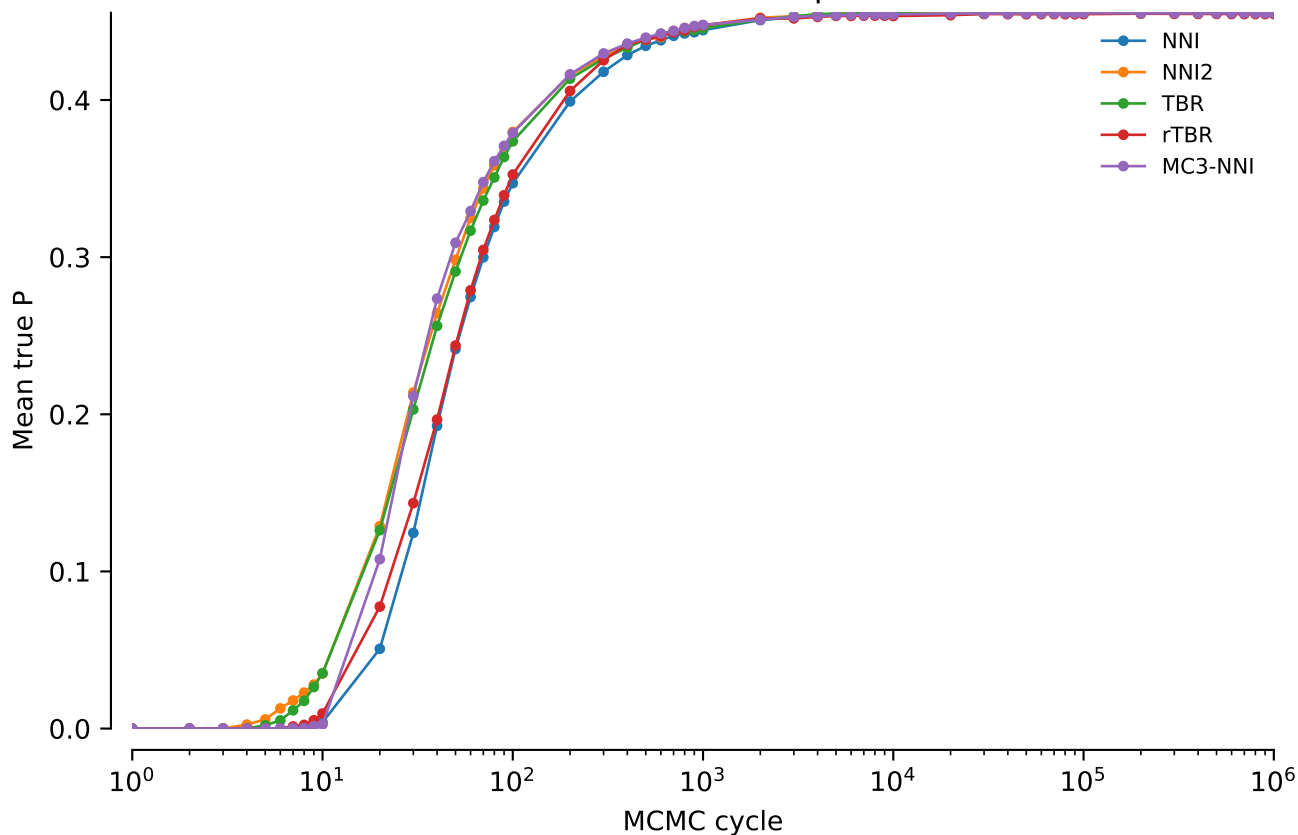
vert.nd1.tw0: Mean true P: power = 0.05
