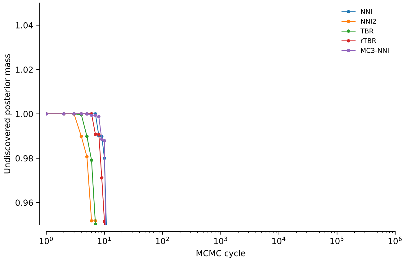
vert.nd1.tw0: Undiscovered posterior mass: power = 0.05
