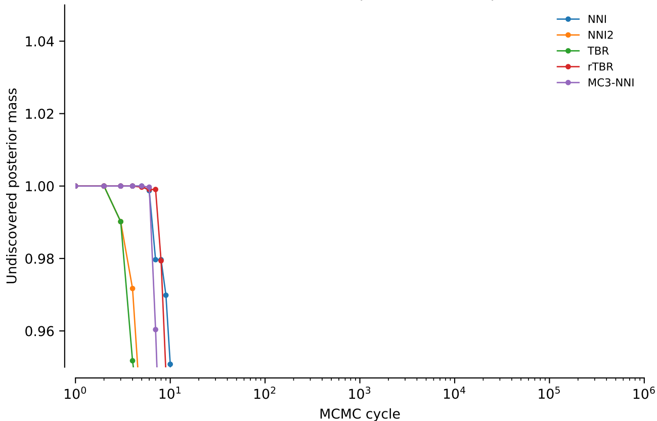
vert.nd1.tw0: Undiscovered posterior mass: power = 0.1
