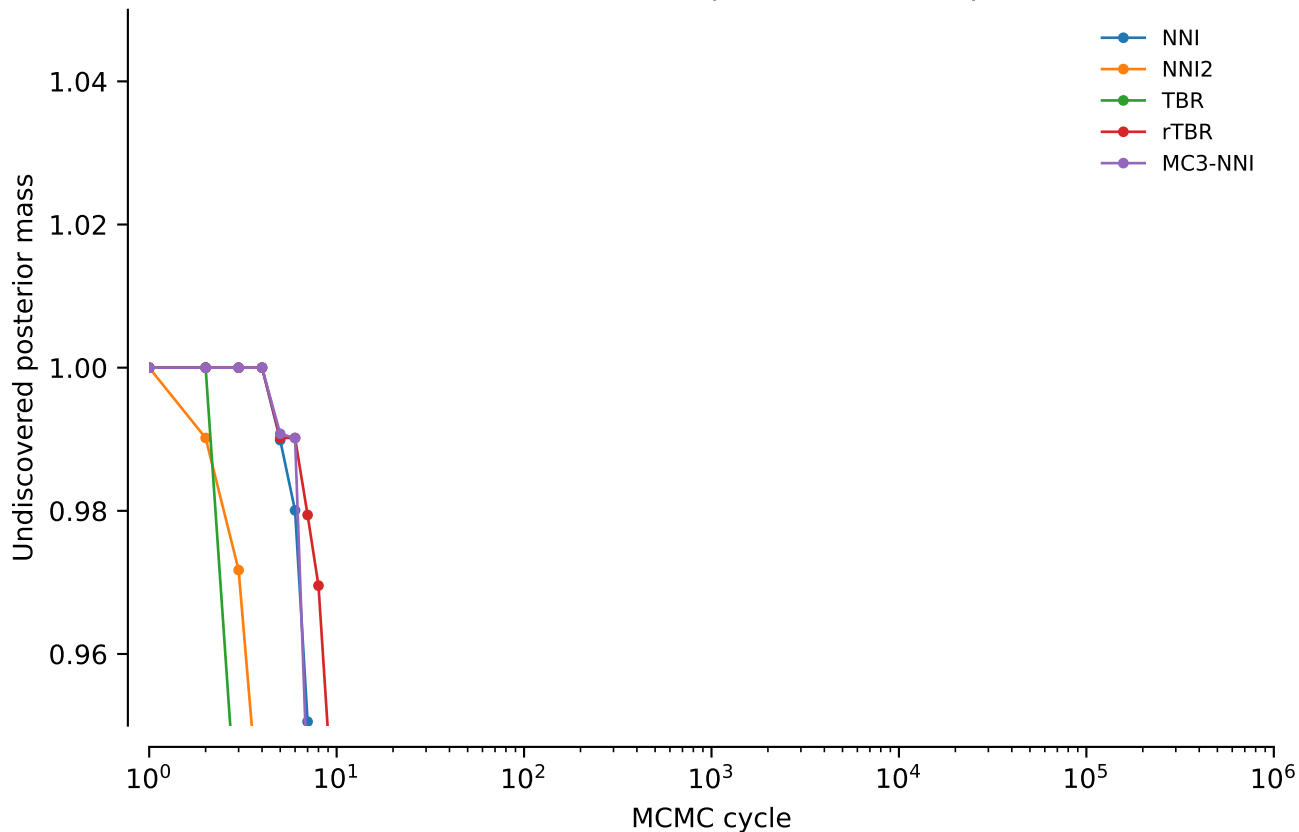
vert.nd1.tw0: Undiscovered posterior mass: power = 0.2
