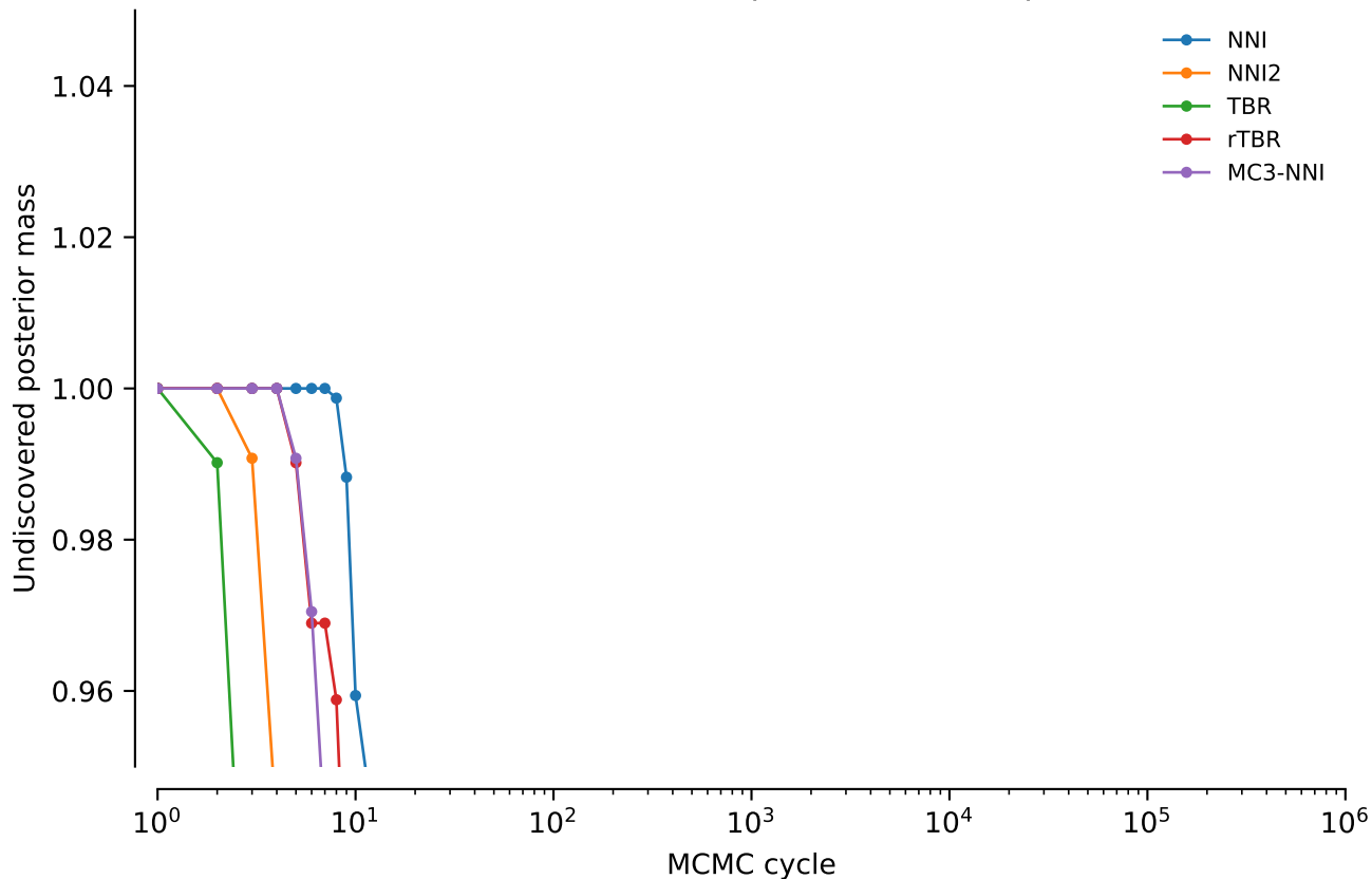
vert.nd1.tw0: Undiscovered posterior mass: power = 0.3
