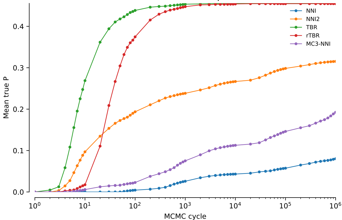
vert.nd1.tw0: Mean true P: power = 0.4
