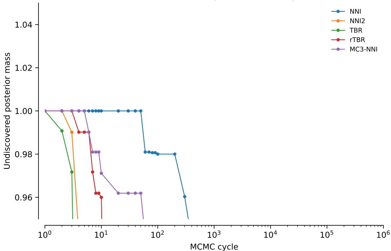
vert.nd1.tw0: Undiscovered posterior mass: power = 0.4
