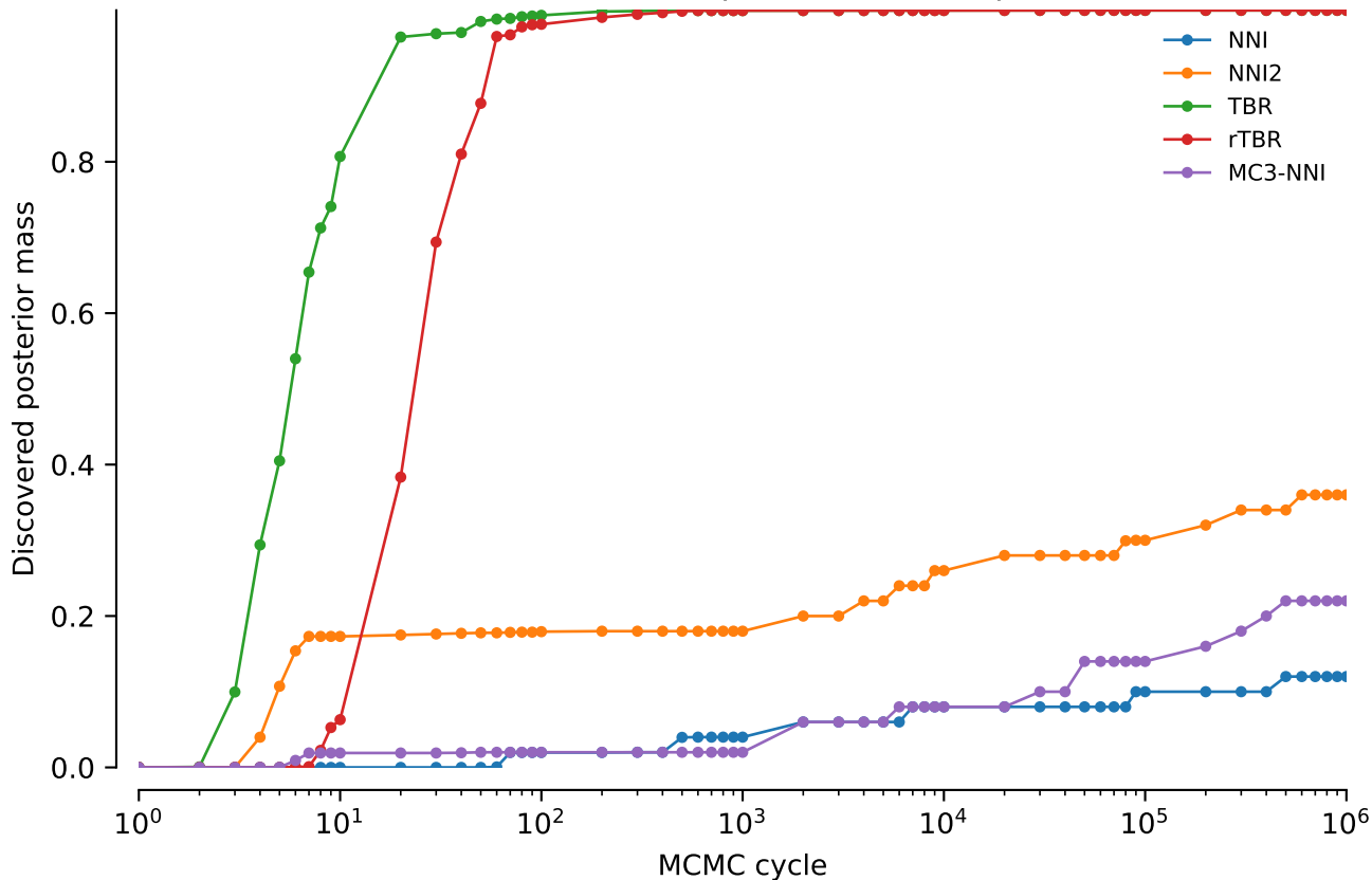
vert.nd1.tw0: Discovered posterior mass: power = 0.5
