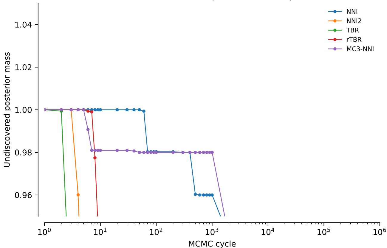
vert.nd1.tw0: Undiscovered posterior mass: power = 0.5
