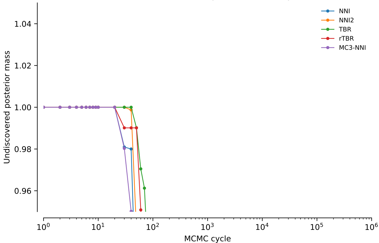
vert.nd1.tw0: Undiscovered posterior mass: power = 0
