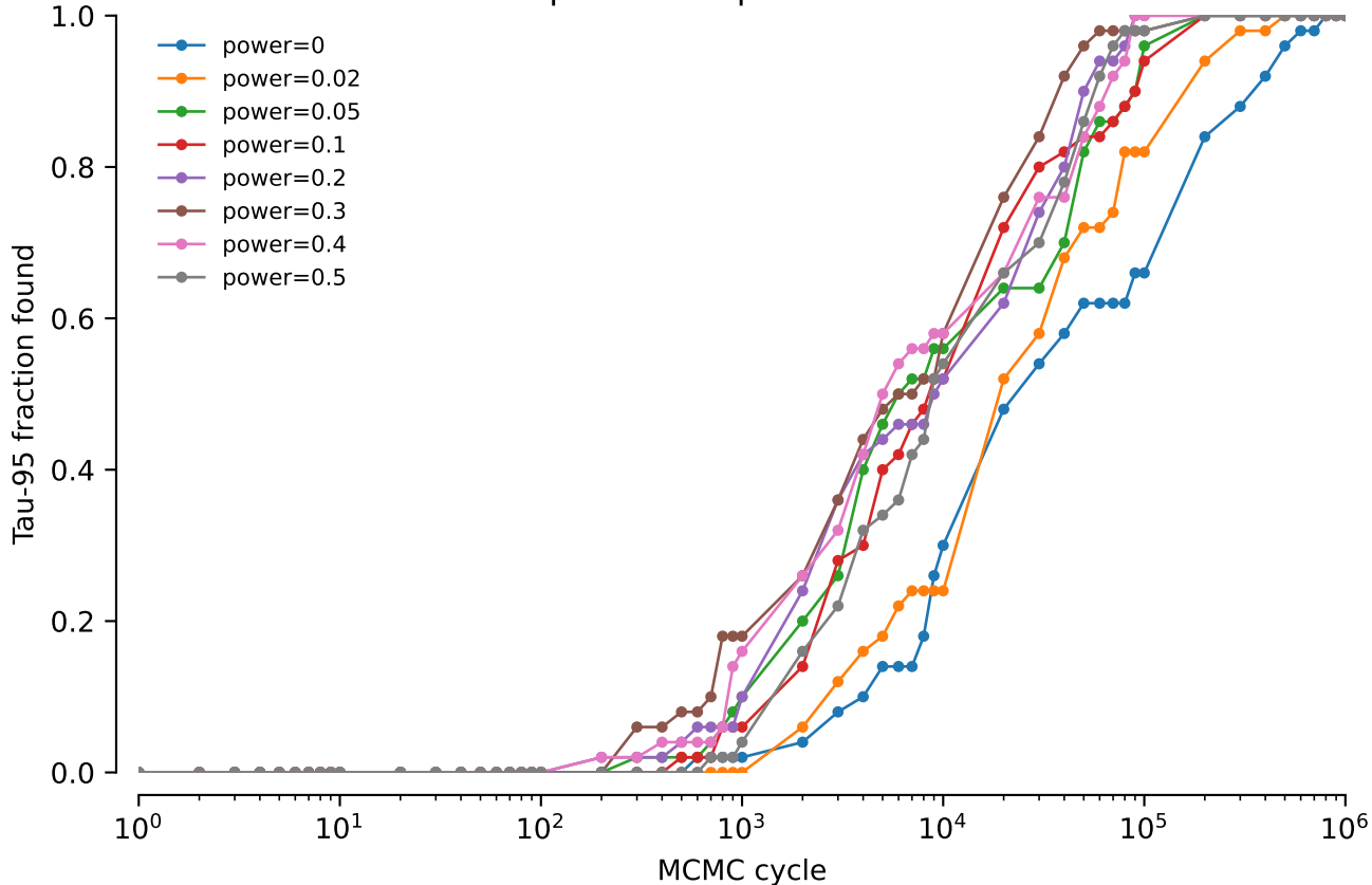
vert.nd1.tw5: NNI power comparison: Tau-95 fraction found
