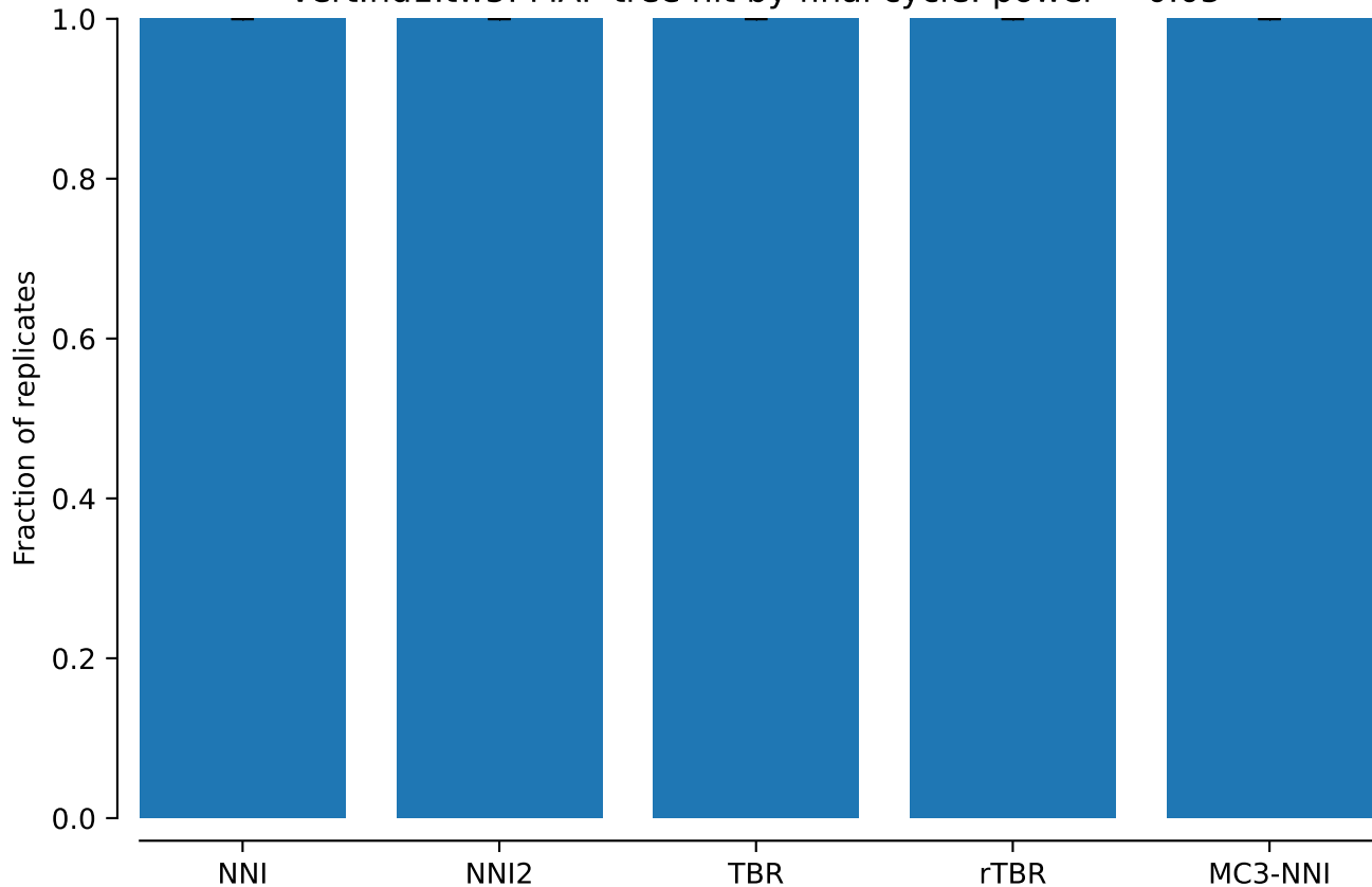
vert.nd1.tw5: MAP tree hit by final cycle: power = 0.05
