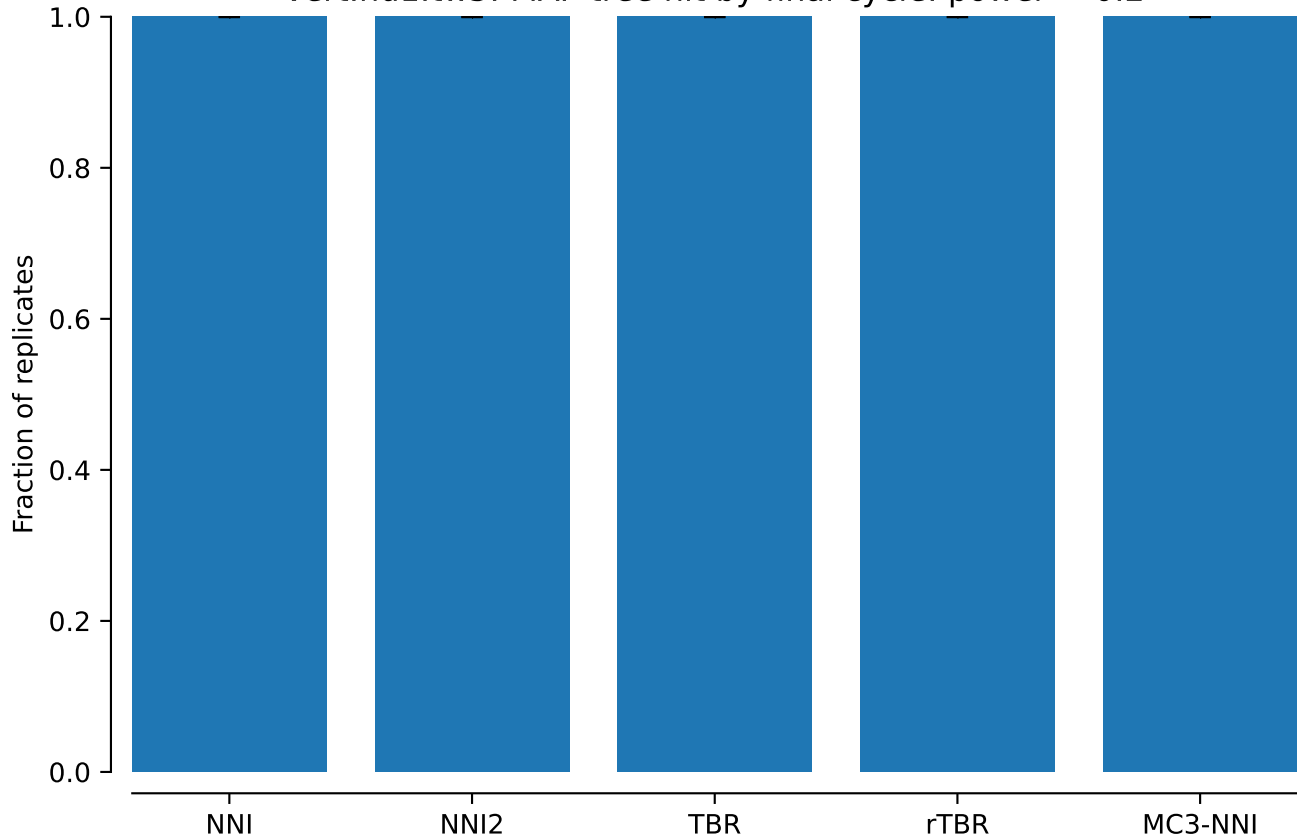
vert.nd1.tw5: MAP tree hit by final cycle: power = 0.2
