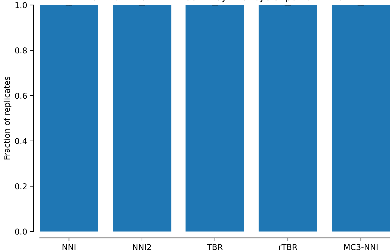
vert.nd1.tw5: MAP tree hit by final cycle: power = 0.5
