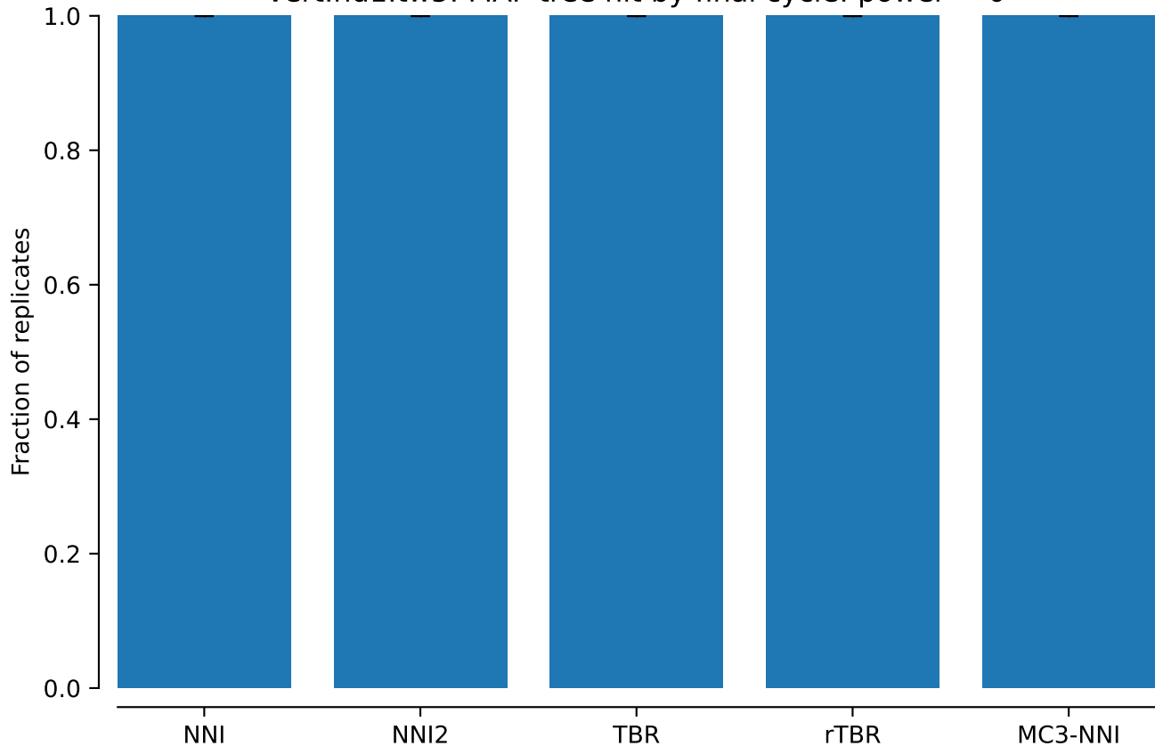
vert.nd1.tw5: MAP tree hit by final cycle: power = 0
