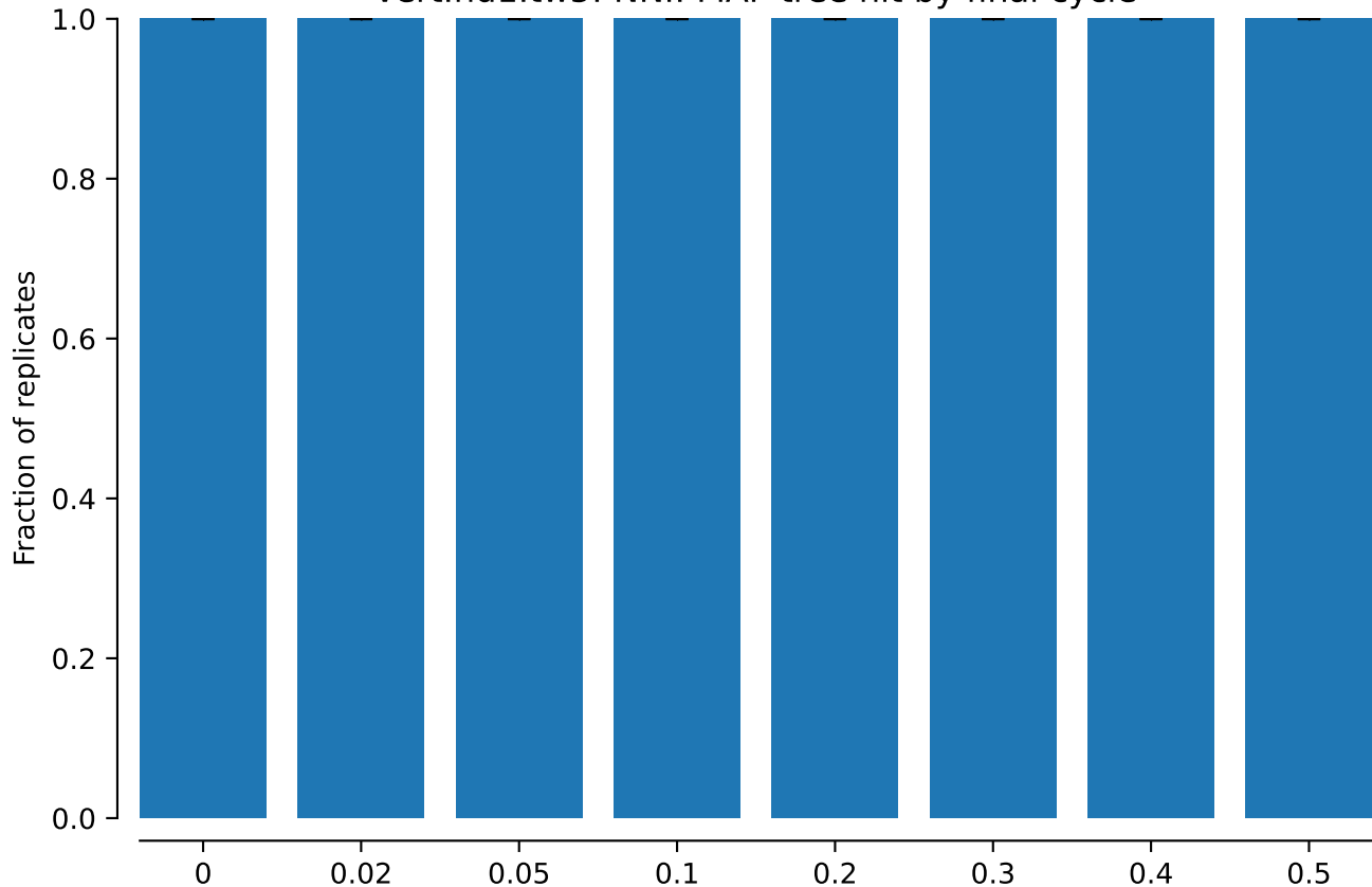
vert.nd1.tw5: NNI: MAP tree hit by final cycle
