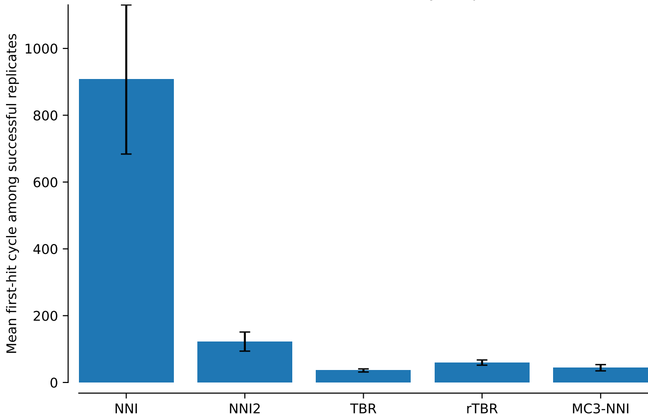
vert.nd1.tw5: Mean MAP first-hit cycle: power = 0.2
