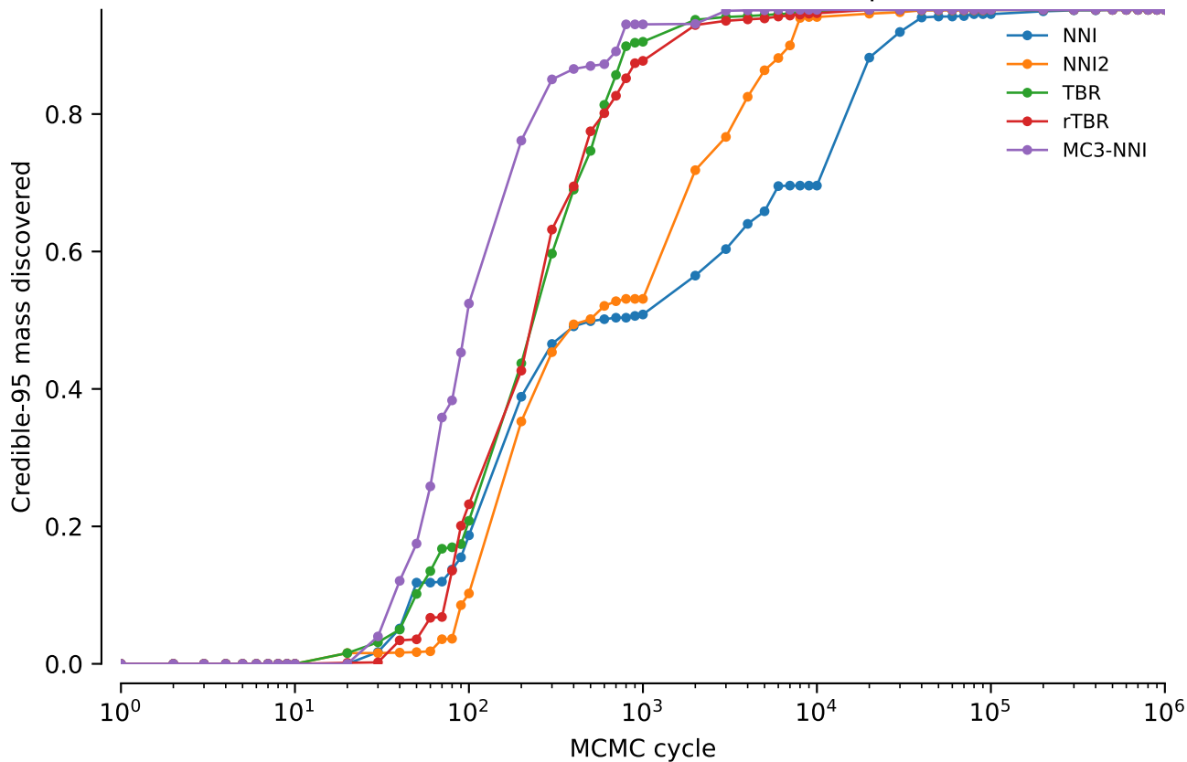
vert.nd1.tw5: Credible-95 mass discovered: power = 0.02
