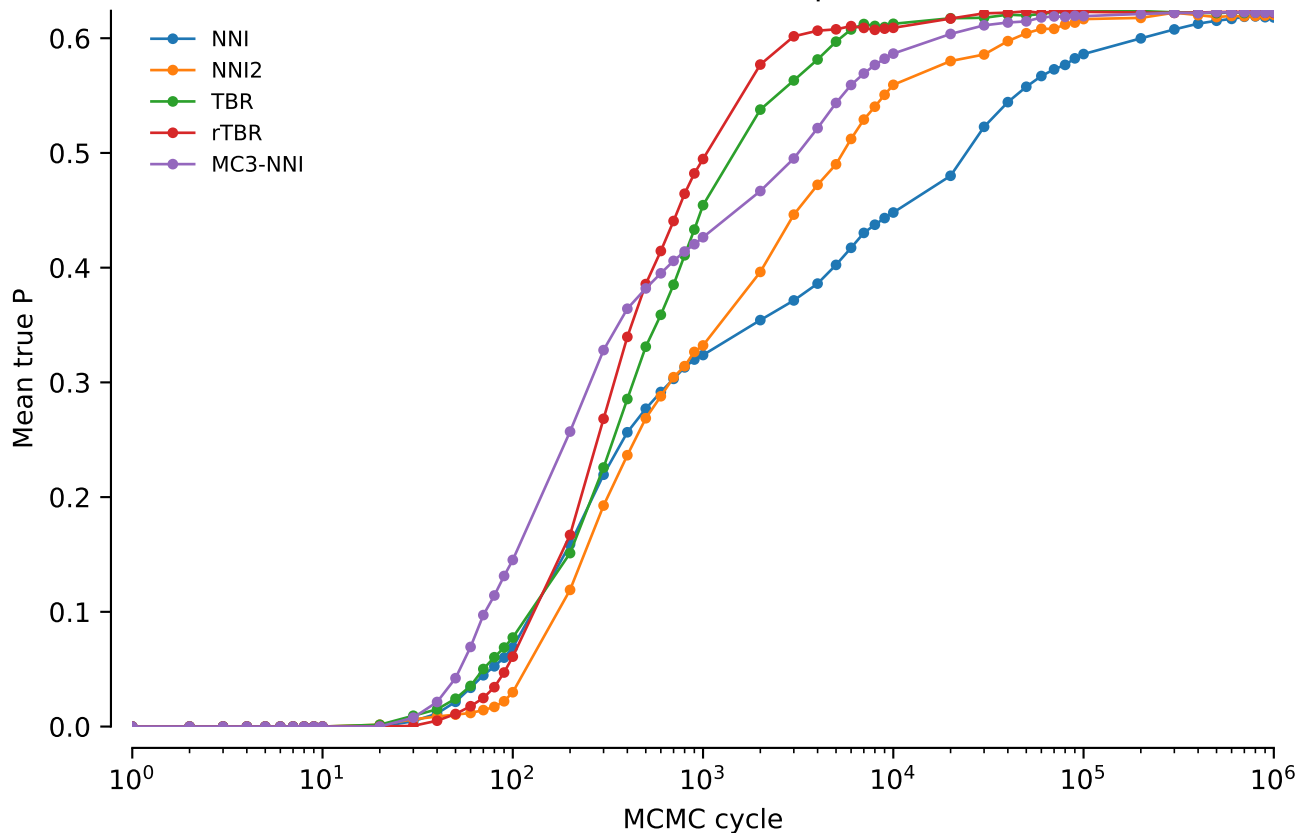
vert.nd1.tw5: Mean true P: power = 0.02
