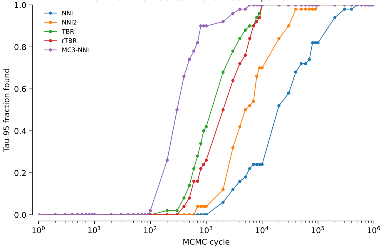
vert.nd1.tw5: Tau-95 fraction found: power = 0.02
