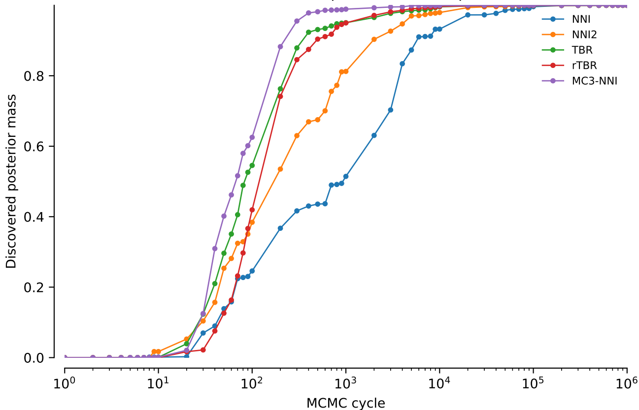
vert.nd1.tw5: Discovered posterior mass: power = 0.05
