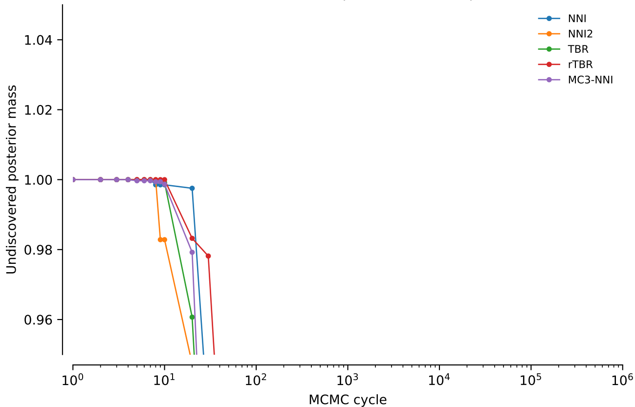
vert.nd1.tw5: Undiscovered posterior mass: power = 0.05
