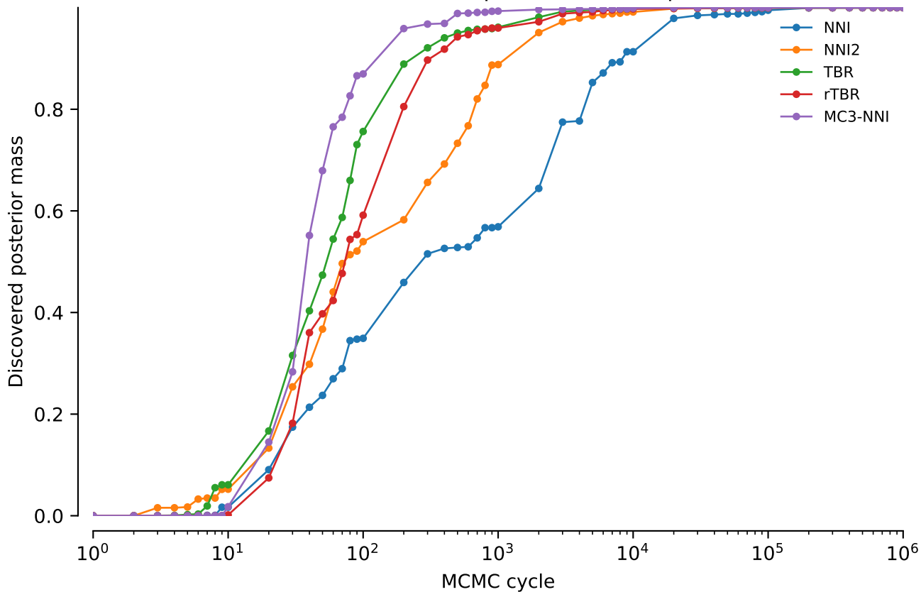
vert.nd1.tw5: Discovered posterior mass: power = 0.1
