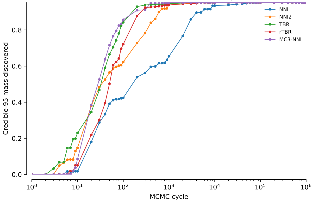
vert.nd1.tw5: Credible-95 mass discovered: power = 0.2
