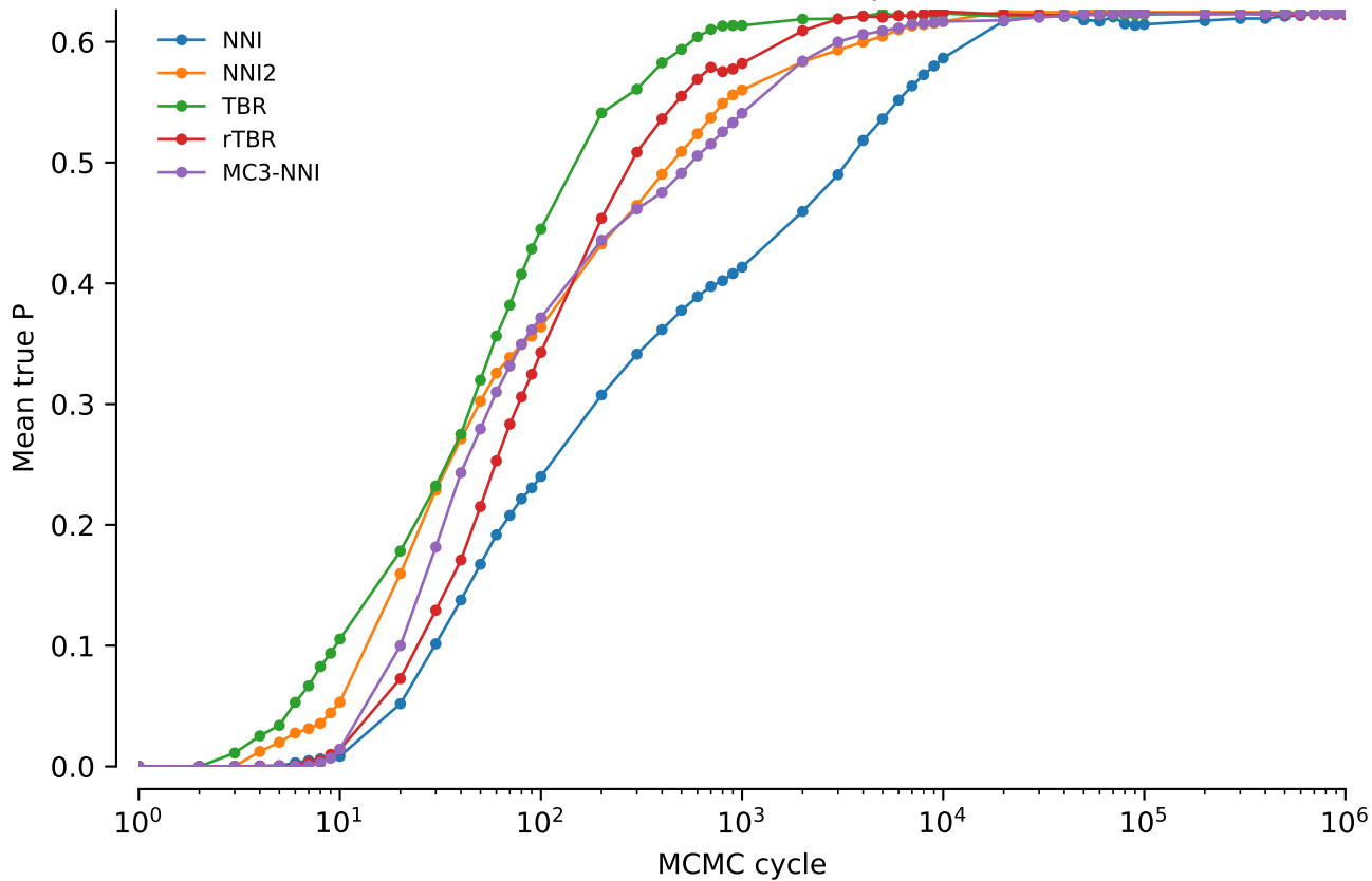
vert.nd1.tw5: Mean true P: power = 0.2
