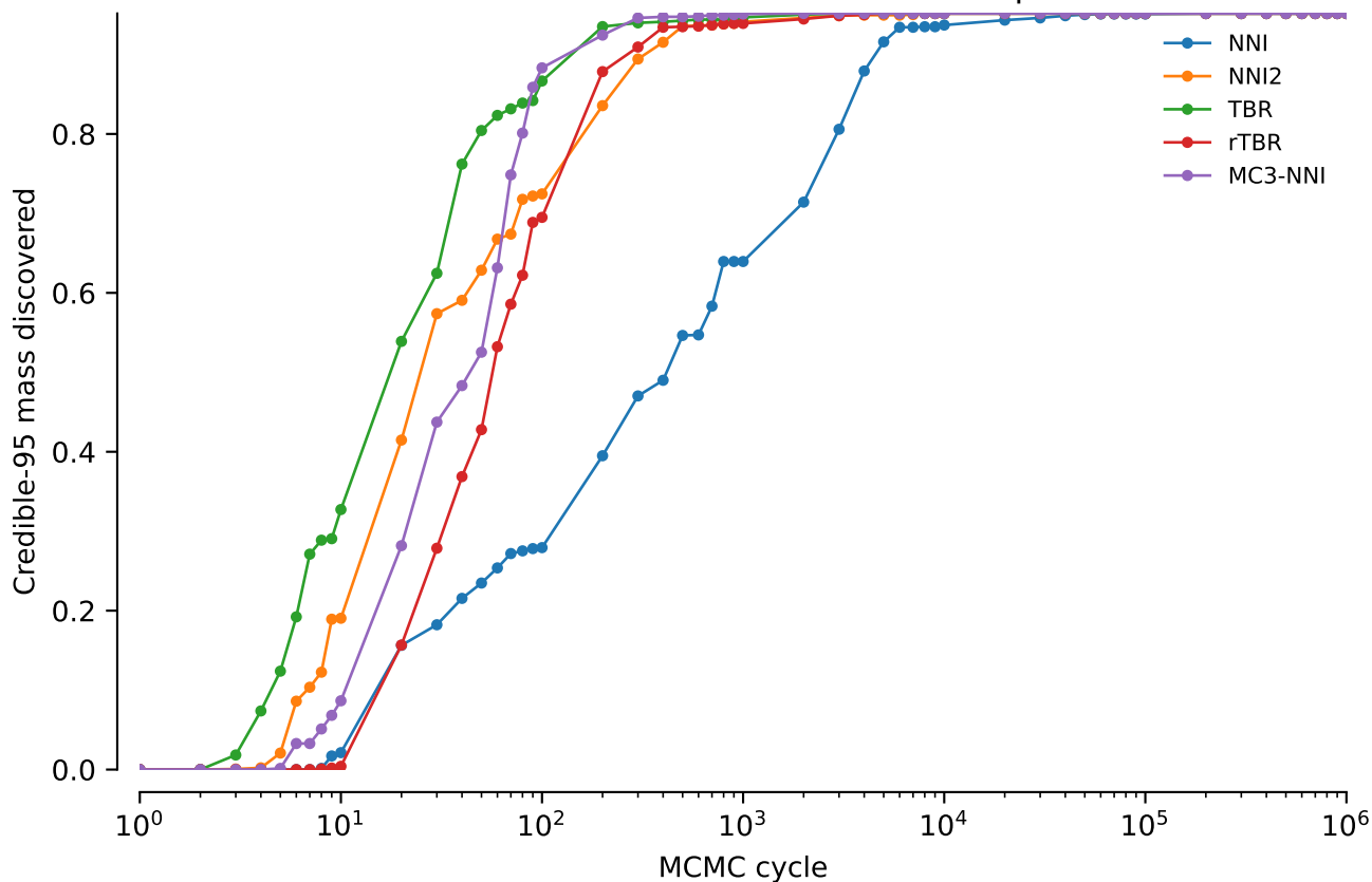
vert.nd1.tw5: Credible-95 mass discovered: power = 0.3
