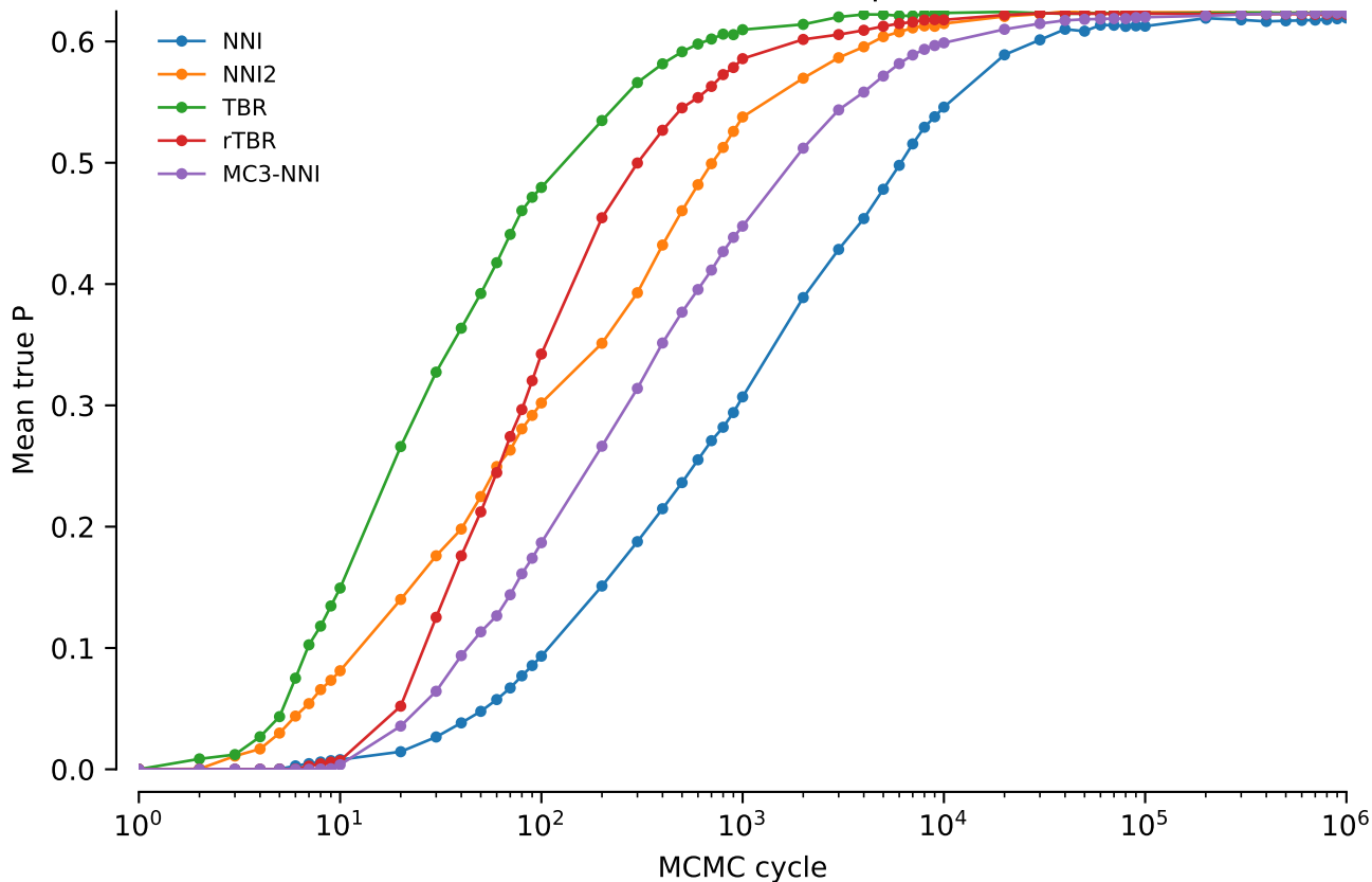
vert.nd1.tw5: Mean true P: power = 0.4
