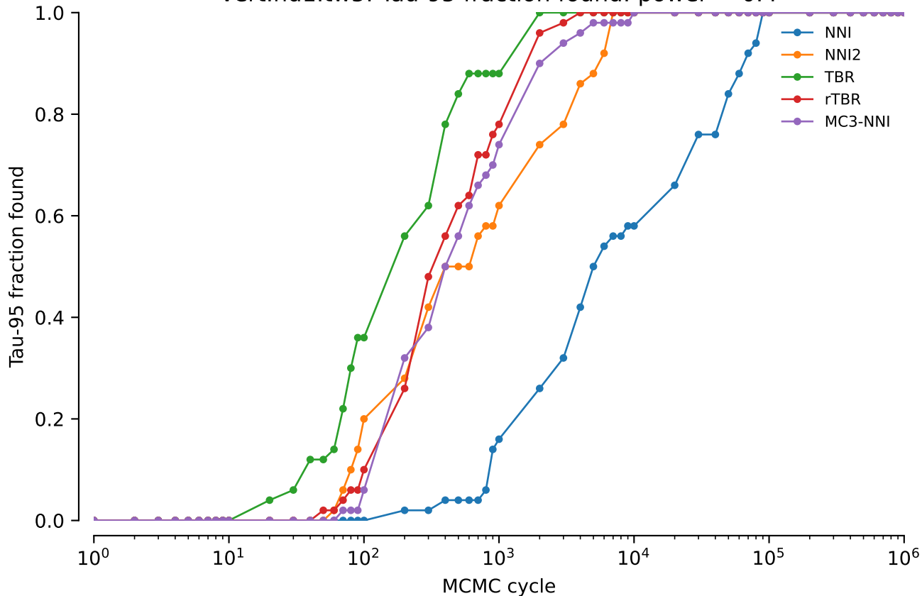
vert.nd1.tw5: Tau-95 fraction found: power = 0.4
