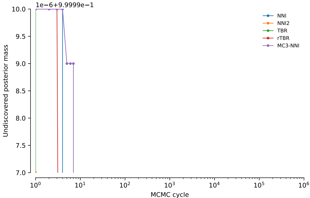
vert.nd1.tw5: Undiscovered posterior mass: power = 0.4
