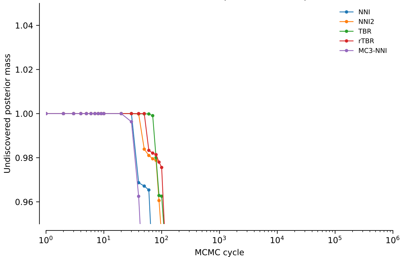
vert.nd1.tw5: Undiscovered posterior mass: power = 0
