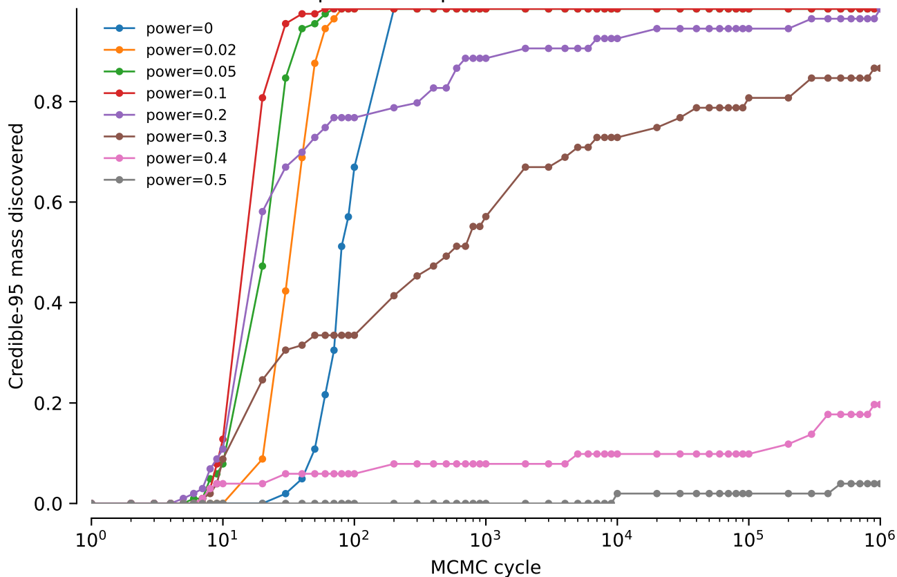
vert.nd2.tw0: NNI power comparison: Credible-95 mass discovered
