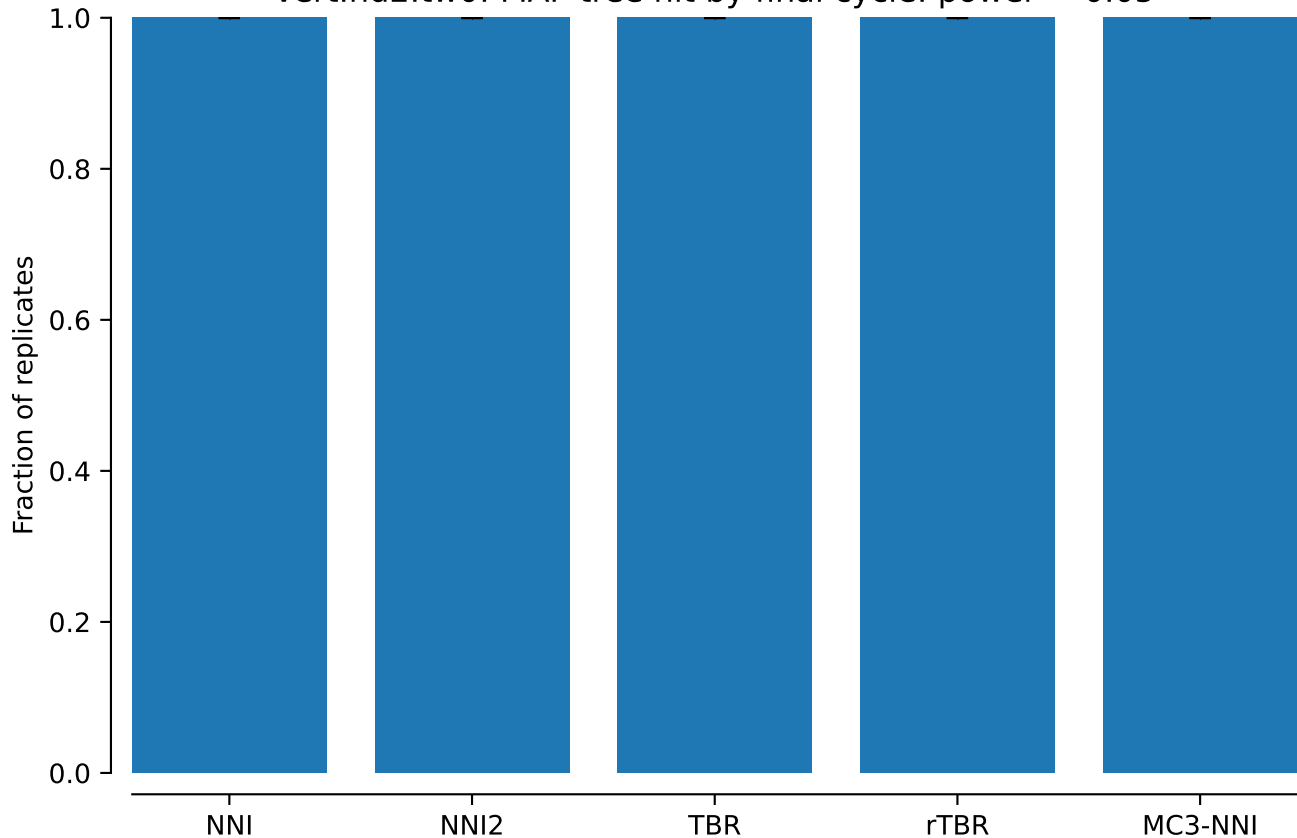
vert.nd2.tw0: MAP tree hit by final cycle: power = 0.05
