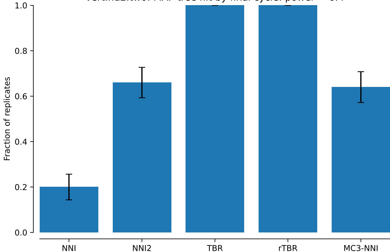
vert.nd2.tw0: MAP tree hit by final cycle: power = 0.4
