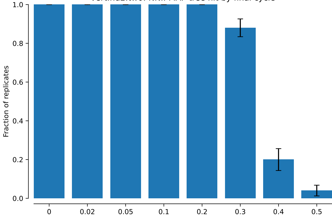
vert.nd2.tw0: NNI: MAP tree hit by final cycle
