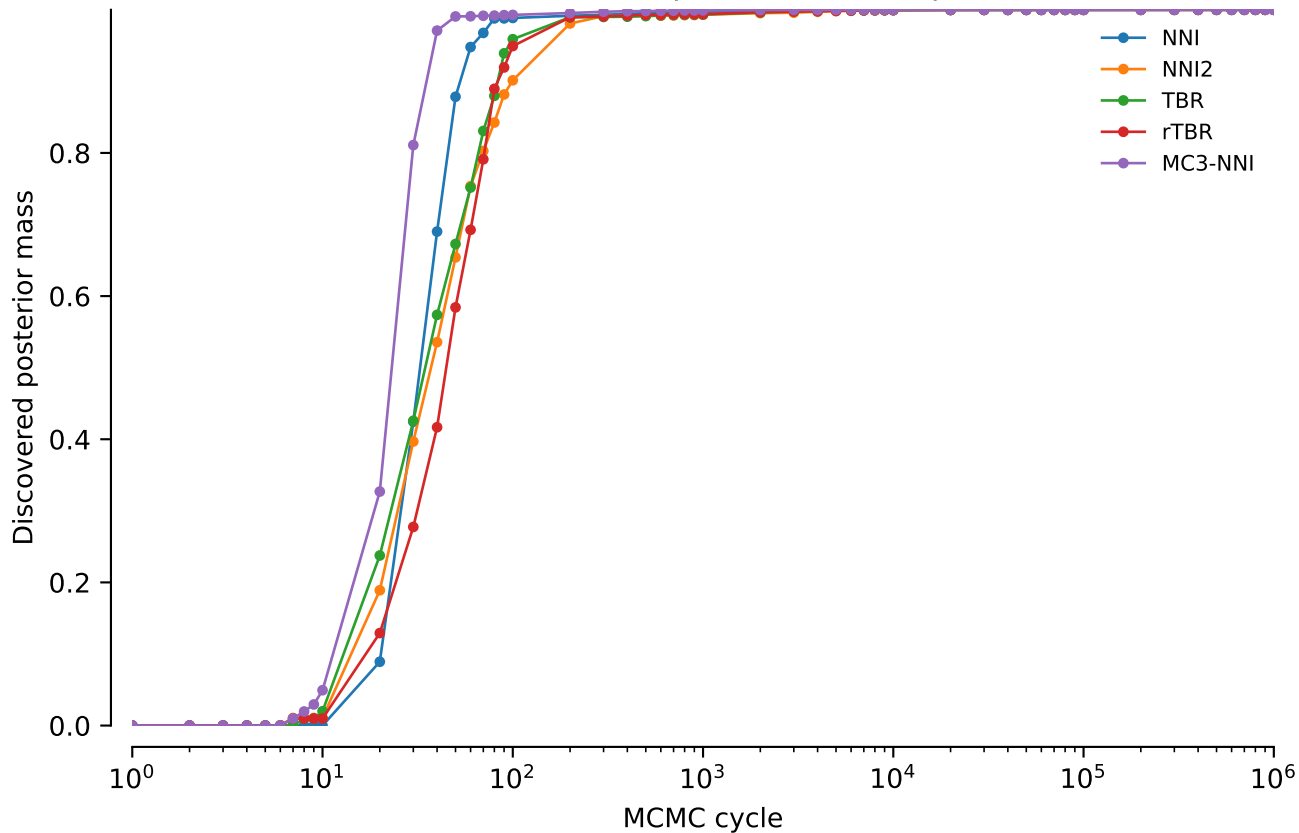
vert.nd2.tw0: Discovered posterior mass: power = 0.02
