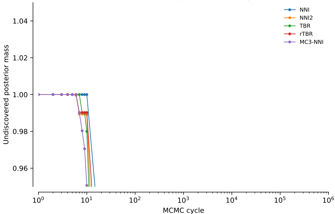
vert.nd2.tw0: Undiscovered posterior mass: power = 0.02
